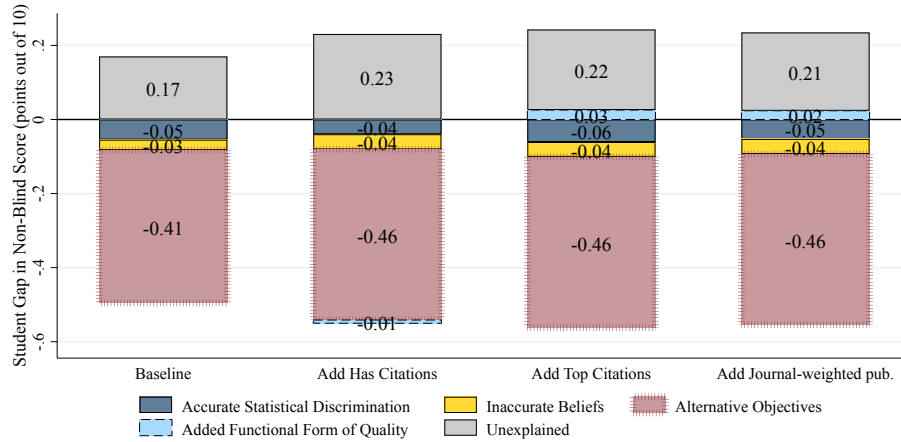
Figure A25: Incorporating Additional Functional Forms of Quality
